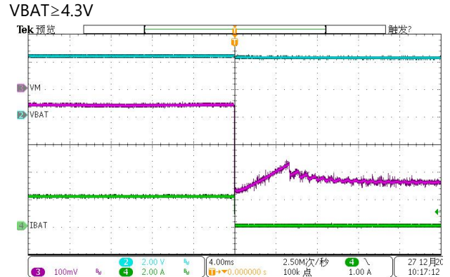
Battery Charging OVP
