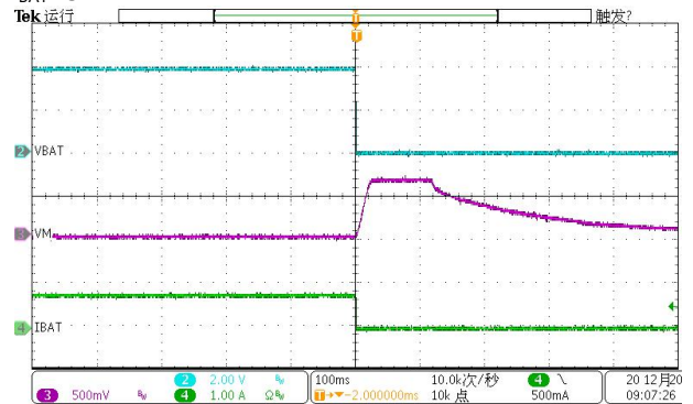
Battery Charging Off
