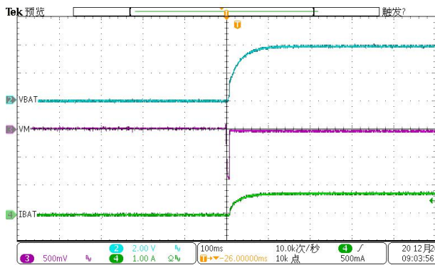
Batter Charging On
