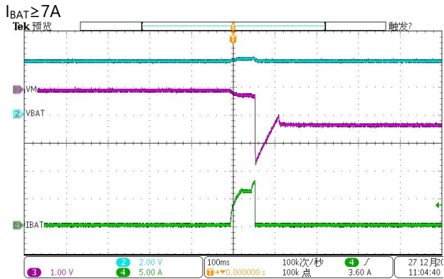
Batter Charging, OCP
