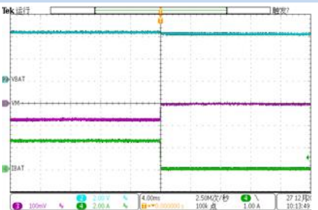
Battery Charging Off
