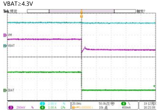
Battery Charging OVP
