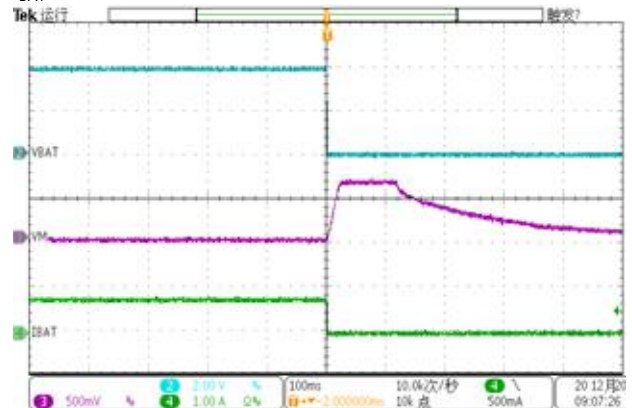
Battery Charging Off
