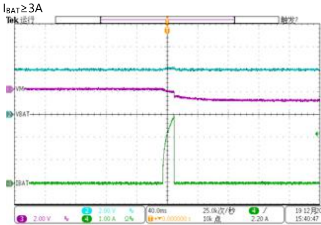
Batter Charging, OCP
