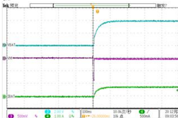
Batter Charging On
